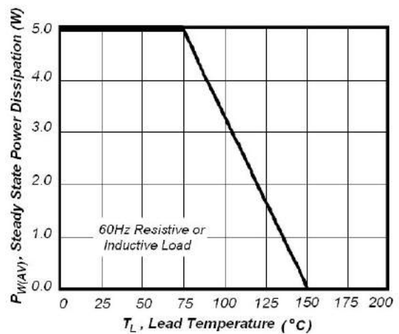
Fig6. Steady State Power
