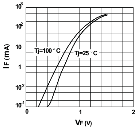
Forward characteristics
